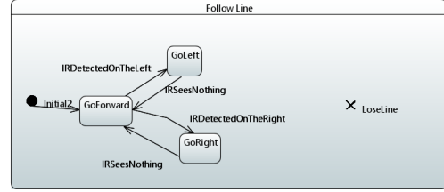
Fig. 14. FollowLineStateMachine
