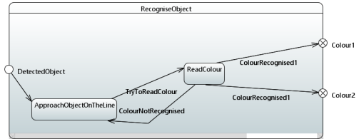
Fig. 15. Recognise Object State Machine
